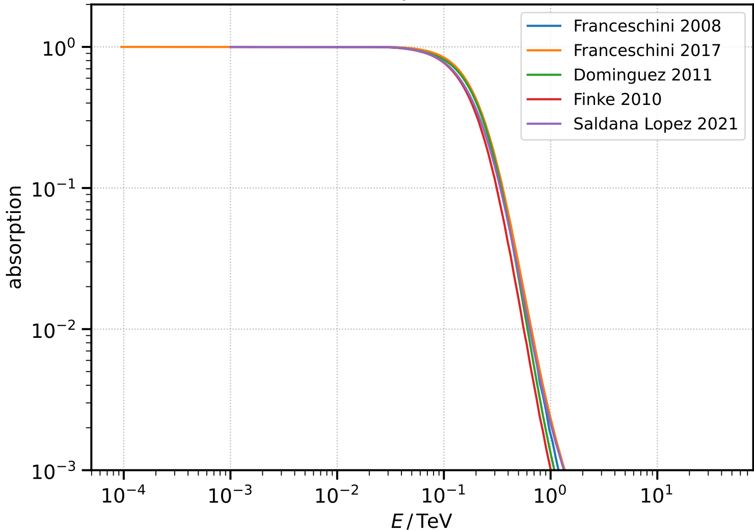
EBL absorption at z=0.5
